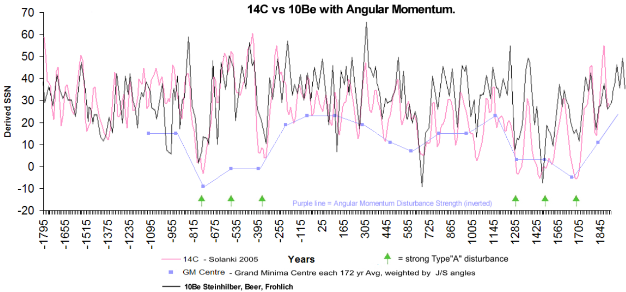
Figure 4. Comparison of 14C and 10Be isotope records. The purple line is a representation of the AMP group strength (individual AMP events are summed to form group totals, details follow in later section) with each point representing the AMP centre. A full size image can be viewed at http://www.landscheidt.info/images/solanki_sharp.png the isotope plots are a graphical comparison of Solanki et al (2004) & Steinhilber et al (2009)
