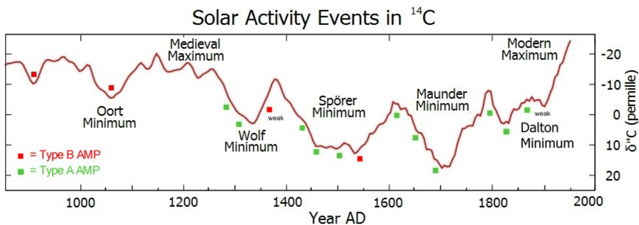
Figure 9. Carbon 14 graph (Wikipedia) with the AMP events overlaid. The Spörer Minimum displaying the longest period of solar inactivity coinciding with 3 strong Type A events and 1 Type B event. The last two AMP events during the Maunder Minimum being stronger than the initial AMP event. See Figure 1&8.
