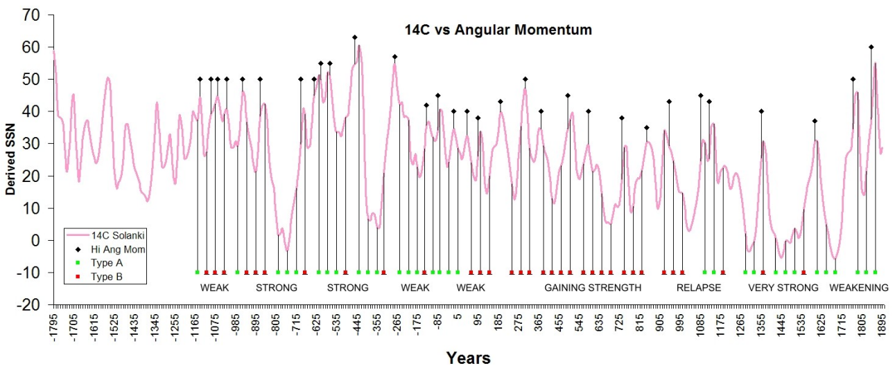
Figure 7. Individual AMP events plotted directly onto the Solanki data. As each conjunction of Uranus & Neptune has a varying Jupiter/Saturn position, the strength of each individual AMP event along with the AMP group total changes over the millennia. This can be represented as the AM power curve of the Holocene. A full size image can be viewed at http://www.landscheidt.info/images/solanki_sharp_detail.jpg spreadsheet with original Solanki data with AMP events available at http://www.landscheidt.info/images/solanki_sharp.xls
