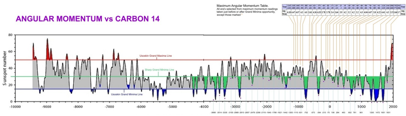
Figure 5. Graphical representation modified from the Usoskin et al. (2007) solar proxy report . Usoskin determining grand minima occur under 15SSN (derived SSN figures) which isolates Dalton Minimum type events. By raising the bar (green line) the repeating pattern of grand minima is observed. The middle AMP event per group shown, the total of the AMP group determining the overall solar downturn of the era. Figure 7 shows each individual AMP event making up each AMP group, the strength of each disturbance coinciding with the relevant planet angles. Type A events with a J/S angle around +30 deg and N/U angle of 15 deg providing the strongest downturns, Type B&A events with a J/S angle near zero deg or 180 deg providing the weakest downturn. A full size image can be viewed at http://www.landscheidt.info/images/c14nujs1.jpg
